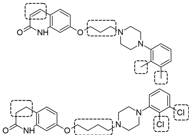
Figure 6. OPC-4392 (top) and aripiprazole (bottom).
