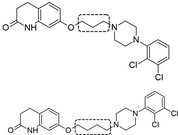
Figure 5. 2,3-dichloro propoxy (top) and aripiprazole (bottom).
